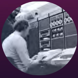
Unix/C/C++
