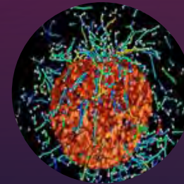
Super-resolution microscopy
